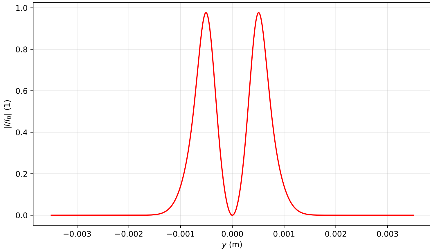
Intensity profile I(x=0, y, z=0.398)/I_0 , \text{Pin}=4.0\text{Pcr} , artificial time
